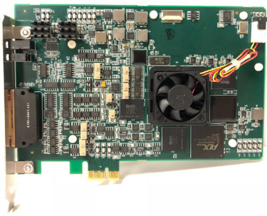
3u 1x channel PCIe
